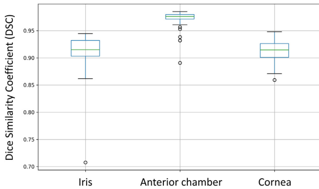
Figure 2. Agreement between ground truth and algorithm-predicted segmentation masks in internal testing.
