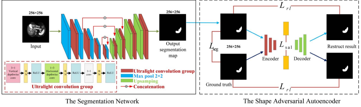
Fig. 2. The overall architecture of SGU-Net. The SGU-Net consists of two parts: the segmentation network on the left and the shape adversarial autoencoder (SAAE) on the right. SAAE encodes both segmentation results and labels into low-dimensional manifold, aiming to constrain their shape representation in low-dimensional manifold. The performance of the segmentation network is improved by adversarial training between SAAE and the segmentation network. It is worth mentioning that SAAE is an additional network that is only used in the training stage, once the training is over, the SAAE will be removed from the testing stage.
