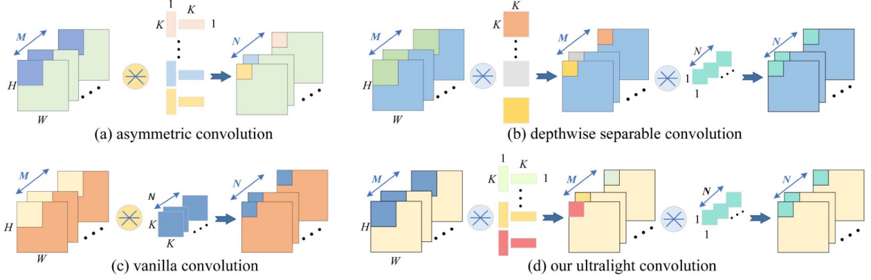
Fig. 3. The comparison between ultralight convolution and popular convolution strategies.
