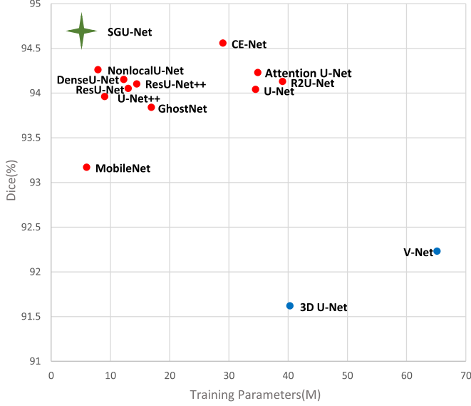
Fig. 1. The Dice value and the number of parameters of different frameworks on CHAOS-CT datasets. Blue points: 3D CNNs. Red points: 2D CNNs. Compared with methods of small memory footprint, the proposed SGU-Net locates in the left-top indicating fewer parameters. while achieving higher performance.
