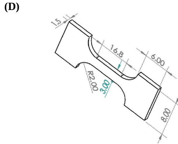
Fig. 1. (A) Scanning strategy for LPBF process of CrCoNi samples. (B) The relative orientation of the compact-tension C(T) and tensile specimens with respect to the build plate, where the Z-axis is parallel to the build direction (BD), the Y-axis to scan direction (SD), and the X-axis to the transverse direction (TD). (C) Dimensions of C(T) sample and (D) tensile specimen dimensions. In Figs. C and D, all the dimensions are in mm.
