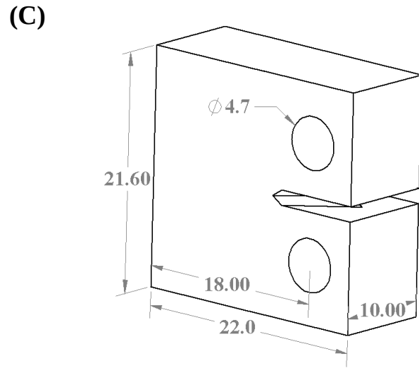
Fig. 1. (A) Scanning strategy for LPBF process of CrCoNi samples. (B) The relative orientation of the compact-tension C(T) and tensile specimens with respect to the build plate, where the Z-axis is parallel to the build direction (BD), the Y-axis to scan direction (SD), and the X-axis to the transverse direction (TD). (C) Dimensions of C(T) sample and (D) tensile specimen dimensions. In Figs. C and D, all the dimensions are in mm.
