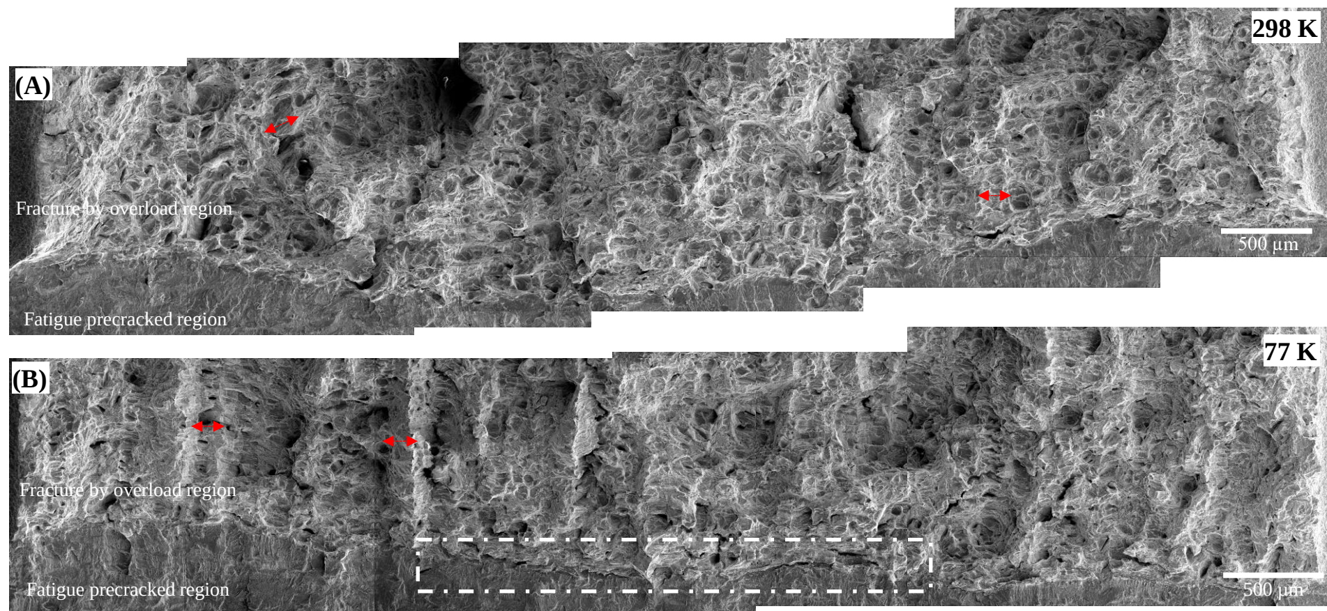
Fig. 8. SEM fractographs showing the tortuosity of the crack path arising from laser scan tracks in specimens tested at (A) 298 K and (B) 77 K. In Fig. (B), the rectangle with white dotted lines shows secondary cracks in the stretch zone, indicating extrinsic toughening. The red double arrow lines show the remanent of laser scan tracks after the fracture.
