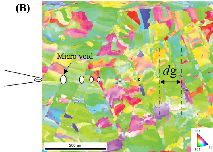
Fig. 9. The stress-state modified critical strain-controlled model for ductile fracture by microvoid coalescence. (A) The plot shows the HRR solutions for the plastic stain, \epsilon_p , distribution at a distance x ahead of the crack tip for a particular crack-tip opening displacement, \delta , in a nonlinear elastic power-law hardening material. The criterion is relevant to the fracture of the CrCoNi by microvoid coalescence; it requires that the local plastic strain \bar{\epsilon}_p exceeds a fracture strain \bar{\epsilon}_f over a characteristic distance, l_0^* , which is related to the characteristic microstructural length scale, d_g . The estimation based on the micromechanics model indicates that the laser scan track's width, h is the characteristic microstructural length scale, i.e. , dg \sim h . (B) The IPF map indicating the boundary of the laser scan track as a preferred location for the nucleation of the microvoid.
