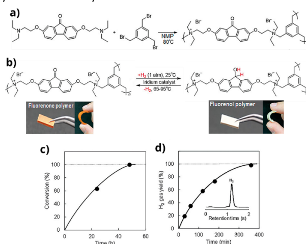
Figure 9. a) Synthesis of Fluorenone polymer, b) dehydrogenated and hydrogenated forms fluorenone (orange)- fluorenel (white) polymer sheets, c) hydrogenation kinetics of fluorenone polymer at 25\text{ }^{\circ}\text{C} and 1\text{ atm} of hydrogen gas and d) dehydrogenation kinetics of fluorenel polymer at 95\text{ }^{\circ}\text{C} (inset gas chromatography plot of hydrogen peak). 52 Copyright Wiley 2020.
