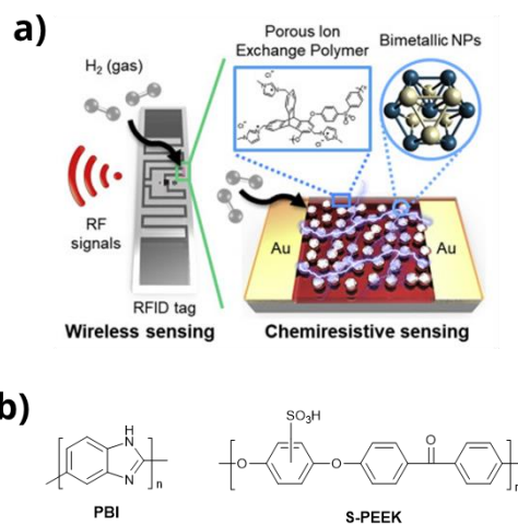
Figure 17. a) Polymer-based RFID sensors (Copyright CelPress 2020), 97 and b) chemical structure of PBI and S-PEEK.
