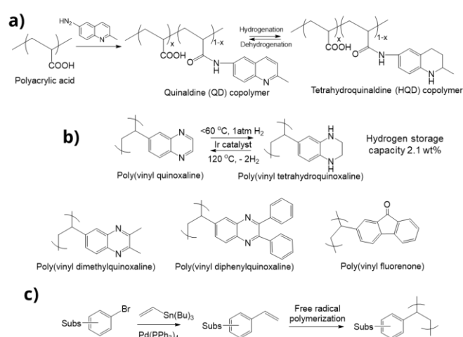
Figure 10. a) Quinaldine copolymer, b) homopolymers from quinoxaline derivatives and fluorenone used for hydrogenation-dehydrogenation studies and c) usual synthesis protocol of monomer and polymer synthesis of quinoxaline and fluorenone.
