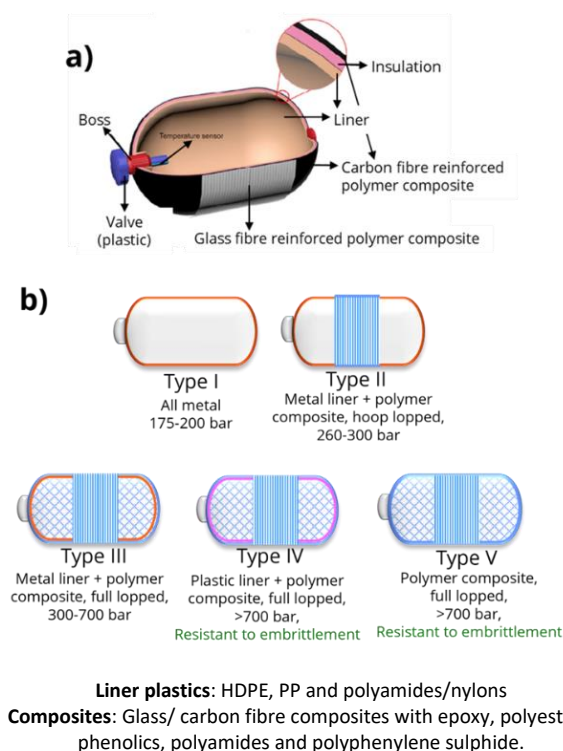
Figure 13. a) General structure of a vehicle on-board high-pressure hydrogen storage tank (copyright ACS 2023), 69 and b) different types of hydrogen storage tanks.
