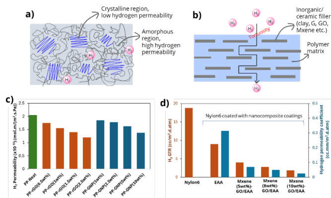
Figure 14. Hydrogen permeability of a) a semi-crystalline polymer and b) a polymer nanocomposite by improving tortuosity. Hydrogen permeability results of c) PP nanocomposite with rGO and GNP, 80a and d) nanocomposite of EAA with GO and MXene. 82
