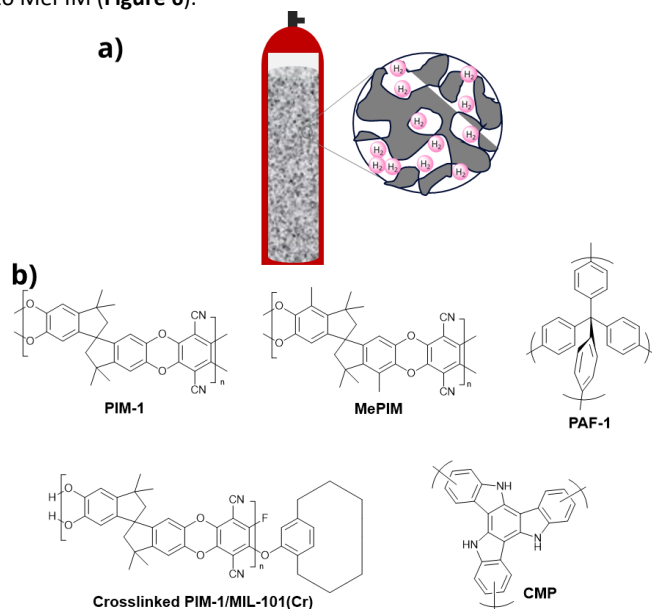
Figure 6. a) Porous polymers for hydrogen storage and b) chemical structure of different polymer of intrinsic microporosity (PIM).
