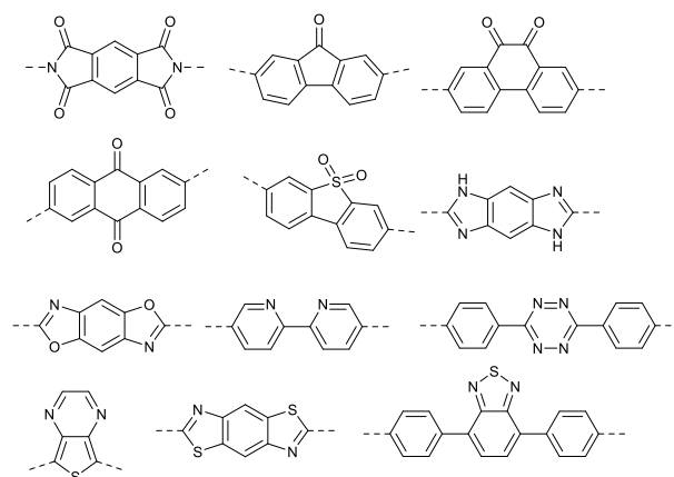
Figure 5. Chemical structure of commonly used polymeric acceptors.
