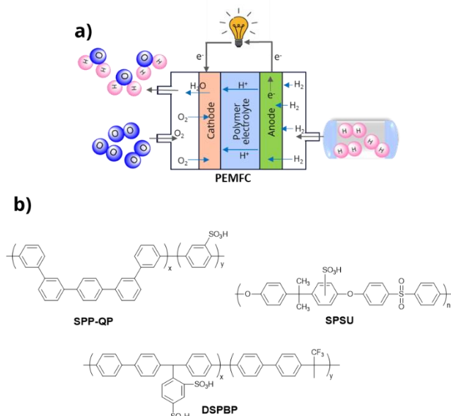
Figure 15. a) A proton exchange membrane fuel cells (PEMFC), and b) chemical structures of some of the sulfonated polymers used as fuel cell membrane.
