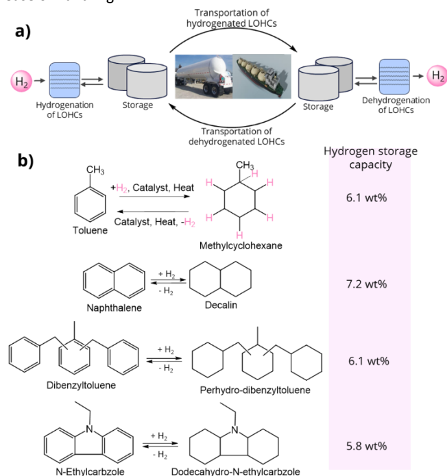
Figure 8. a) Role of LOHCs on hydrogen transportation and b) example of a few common LOHCs in their hydrogenated and dehydrogenated forms.
