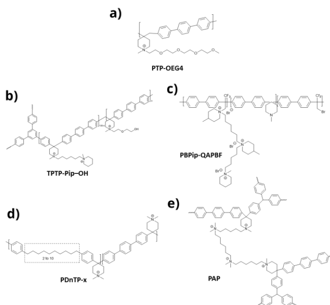
Figure 16. Chemical structure of a) PTP-OEG4, b) TPTP-Pip-OH, c) ether-free fluoropolymer PBIP-QAPBF, d) poly(aryl-co-terphenyl piperidinium) based AEMs PDnTP-x and e) poly(aryl piperidinium) (PAP) based anion exchange membrane.
