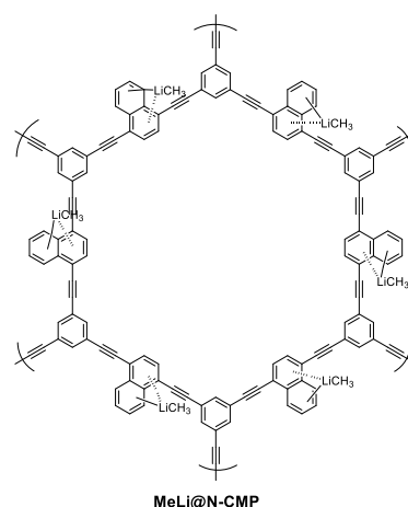
Figure 7. Chemical structure of MeLi@N-CMP.
