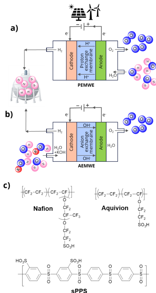
Figure 3. a) proton exchange membrane water electrolyzers (PEMWE), b) anion exchange membrane water electrolyzers (AEMWEs) and c) chemical structure of Nafion, Aquivion and sulfonated poly(phenylene sulfone) (sPPS) used as membrane materials.
