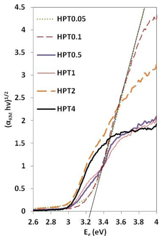
Figure 4. Kubelka-Munk plots of HPT samples.
