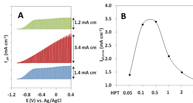
Figure 5 A). Representative photo-voltammograms of selected TiO 2 samples, recorded between -1.1 V and 0.5 V, in 0.1 M Na 2 SO 3 , at a sweep rate of 2 mV s -1 using a 300W Hg-Xe arc lamp. B) Comparison of the maximum photocurrent values obtained for the various TiO 2 samples.
