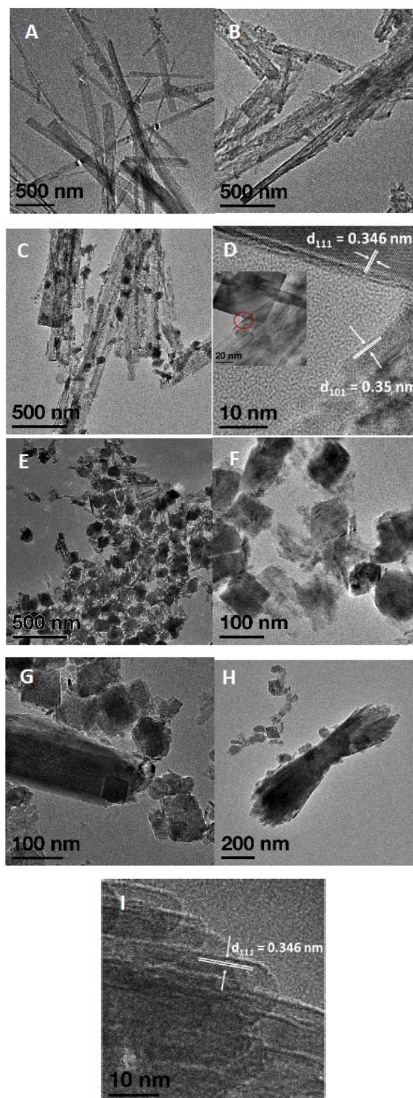
Figure. 2. TEM images of A) as-prepared H-TNFs, B) HPT0.05, C) HPT0.1, D) HRTEM image of HPT0.1; inset shows the area marked by red circle E) HPT0.5, F) HPT1, G) HPT2, and H) HPT4 \text{TiO}_2 products I) HRTEM of HPT4
