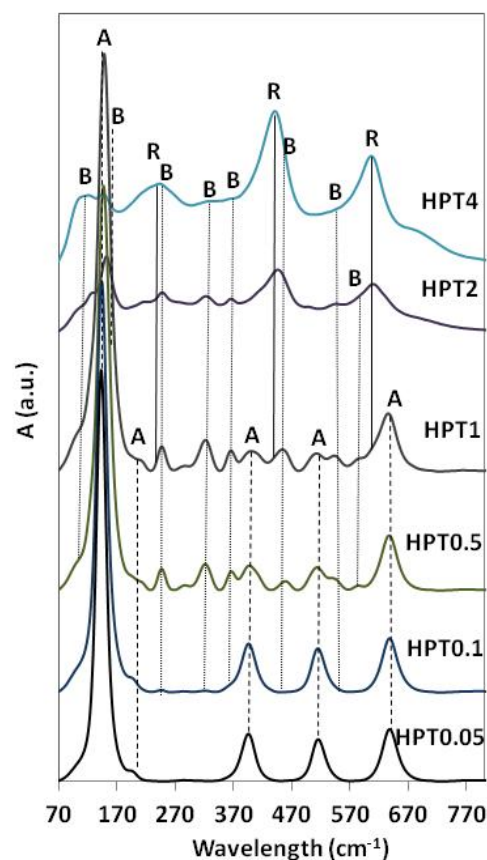
Figure 3. Raman spectra of HPT TiO 2 samples. A, B and R are referring to the representative vibrations of anatase, brookite, rutile, respectively.
