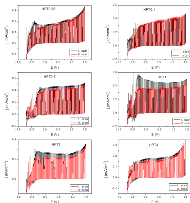
Figure 6. Different decaying behaviours of the photocurrents of the \text{TiO}_2 samples assessed by consecutive photovoltammetric scans. The scans were recorded between -0.7 V and 1.5 V, in 0.1 M \text{Na}_2\text{SO}_4 , at a sweep rate of 2 \text{ mV s}^{-1} using a 300W Hg-Xe arc lamp.
