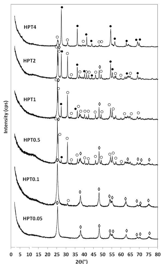
Figure 1. XRD patterns of HPT \text{TiO}_2 samples: ◇ Anatase; ○ Brookite; ● Rutile
