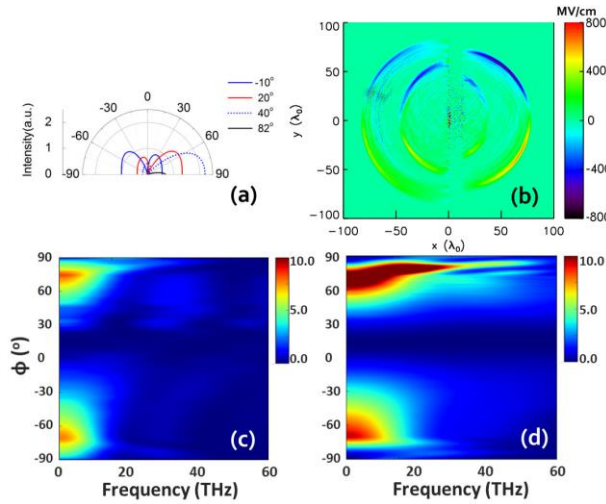
Figure 1. (a) Angular distribution of TR from a single electron by the theory model of eq. (2). Incidence angle of electron is marked with lines of different color. PIC Simulations of laser-solid plasma target interaction: (b) Snapshot of electric field E_y ; Spectrum of the (c) backward (reflected) and (d) forward (transmitted) radiations. Laser duration is 80 fs, peak intensity 7.7 \times 10^{17} W/cm 2 , spot size 4 \mu\text{m} , incidence angle 30°.
