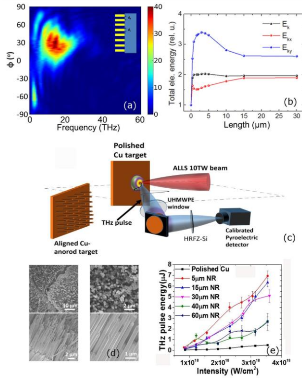
Figure 2. THz radiation generated from nanorod targets. PIC simulation results: (a) Spectrum of reflected radiation, inset is the schematic of the target; (b) Total electron energy as a function of nanorod length h . h=4\ \mu\text{m} in (a). laser duration is 40 fs, peak intensity 3.5 \times 10^{18}\ \text{W}/\text{cm}^2 . Experiment results: (c) Schematic of the experimental setup; (d) SEM images of Cu nanorod arrays; (e) THz pulse energy for different targets as a function of laser intensity. Spacing and width of nanorods are d_0=d_1=0.2\ \mu\text{m} in simulations and experiments.
