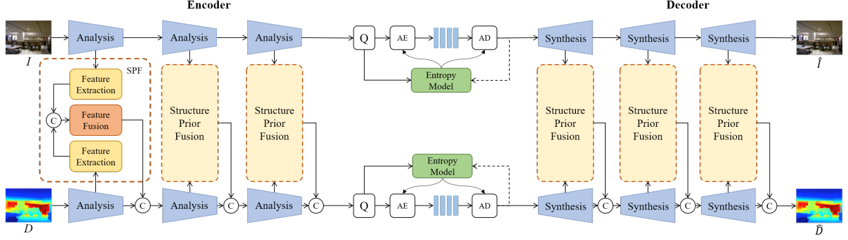
Fig. 2. An example architecture of our proposed depth map compression framework with three pairs of SPF modules. The structure information is extracted by Feature Extraction blocks and fused in Feature Fusion block.
