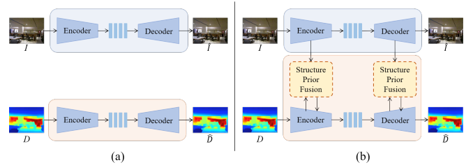
Fig. 1. The overview of the traditional RGB-D compression pattern and our proposed framework. (a) Traditional RGB-D compression pattern; (b) Enhanced depth map compression with RGB-to-Depth structure priors.
