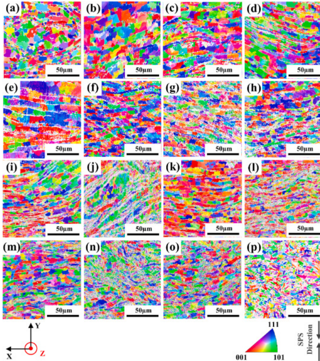
Fig. 5. Crystallographic texture maps of Fe-xCu alloys taken out-of-plane (Z direction), (a)–(p) represent the Cu content of 1, 2, 3, 4, 5, 6, 7, 8, 9, 10, 15, 20, 25, 30, 35 and 40 wt.%, respectively.
