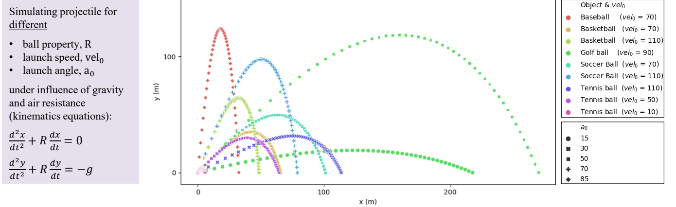
Fig. 6: Example of learning PINN for simulating a distribution of tasks with a priori unknown input conditions in a what-if analysis: projectiles of ball with different physics properties and initial conditions (launch angle and launch speed).
