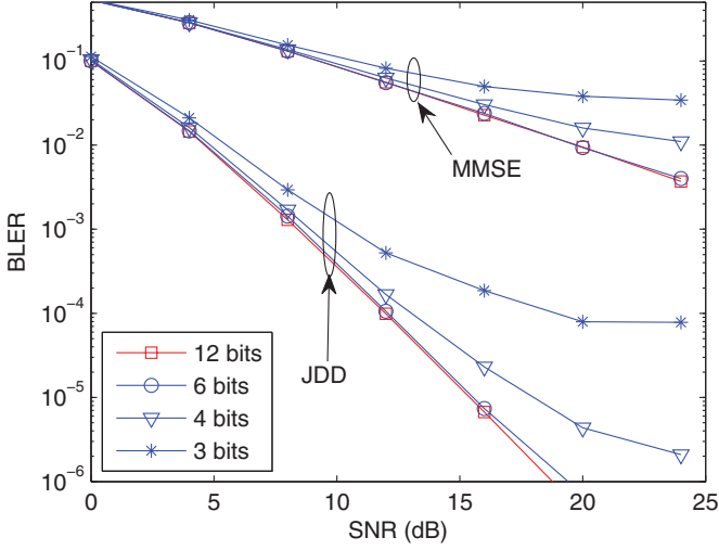
Fig. 2: BLER of the JDD algorithm with different fronthaul sampling resolution Q = 3, 4, 6, 12 bits.
