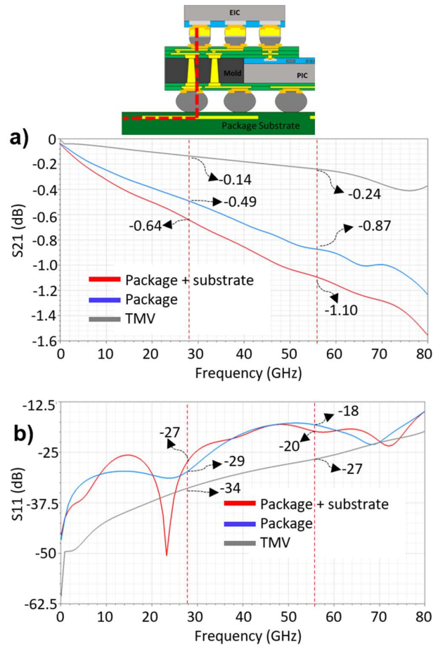
Fig. 3. a) Plot showing the frequency response of the differential transmission interconnects connecting the substrate to the input of the EIC (driver) including the \mu bump, front side RDL, TMV, backside RDL, c4 bump and substrate a) insertion loss b) reflection loss.
