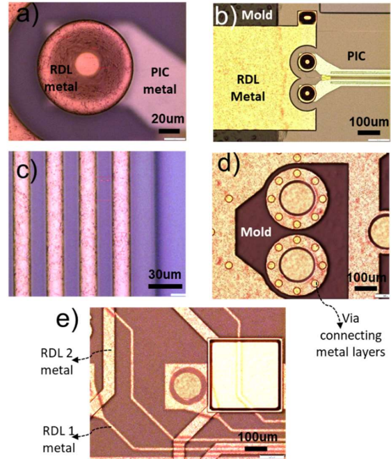
Fig. 9. Images of package RDL processing a) via connecting PIC metal to package RDL metal. b) Metal connecting PIC to the fan-out area. c) Package metal interconnects with line/space of 15 \mu m/15 \mu m. d) high-speed metal interconnects from modulators on mold area. e) image showing RDL 1 and RDL 2 metal.
