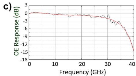
Fig. 6. a) Modulator EO bandwidth b) 100Gbps PAM-4 eye diagrams c) Waveguide germanium photodetector OE bandwidth.
