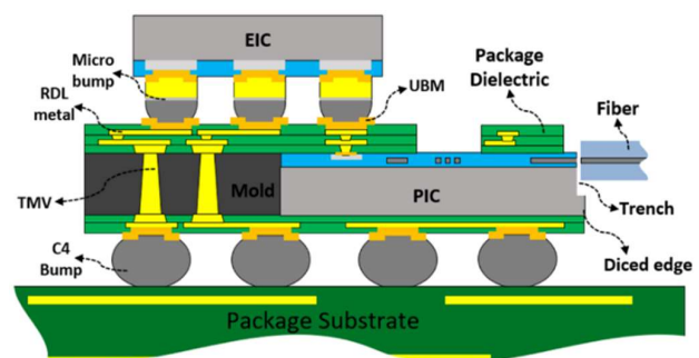
Fig. 1. The cross-sectional layout of the optical engine is realized by fan-out wafer-level packaging. The package contains photonic integrated circuit chips that are encased within an epoxy mold compound and EICs mounted on the surface. The mold area that surrounds the PIC enables electrical routing to the substrate.
