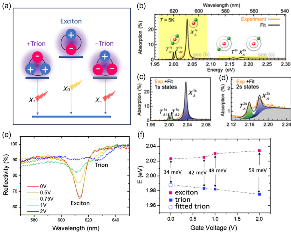
Fig. 2 (a) Illustration of the exciton and trion. (b) Optical absorption spectrum of an h-BN-encapsulated WS 2 monolayer measured at T = 5 K. (c) Experimental and fitted spectra for n = 1 states, where shaded green and blue regions represent the contributions from trions and excitons, respectively. (d) Zoomed-in view highlighting ( n = 2 ) excited state trions and excitons. (e) Cavity-enhanced exciton-trion resonance at RT. (f) WS 2 trion binding energy measured at RT. Panels (b)–(d) were reproduced with permission from Ref. 56 © 2019—APS, and panels (e) and (f) were reproduced with permission from Ref. 58 © 2023—Wiley.
