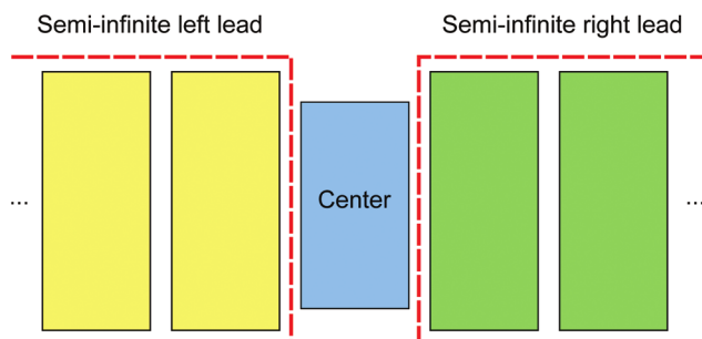
Fig. 1 Schematic of the AGF setup. The finite center (solid blue region), which represents the boundary region, is sandwiched between the semi-infinite left (solid yellow) and right (solid green) leads that represent the lattice bulk regions. The leads can be organized as a semi-infinite periodic array of slices that correspond to the unit cells of the bulk.
