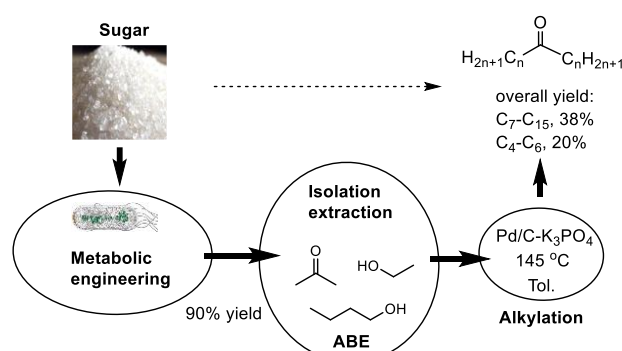
Scheme 1. Conversion of sugars to high-molecular-mass hydrocarbons by the combined metabolic engineering and chemocatalysis process.
