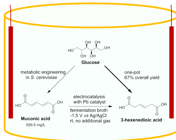
Scheme 3. The sequential fermentation/electrocatalytic reduction of glucose into 3-hexenedioic acid by a combined metabolic engineering and electrocatalysis process in one pot. The selected electrocatalysis step allows using fermentation broth as electrolyte and hydrogen source.
