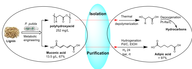
Scheme 2. The combining of metabolic engineering and chemocatalysis for lignin upgrading to hydrocarbons and adipic acid.
