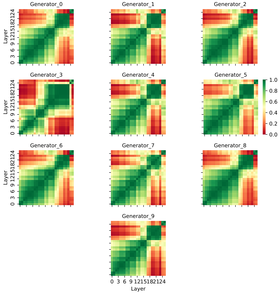
Fig. 3: Linear CKA between layers of individual searched generator networks by DONAS-GAN for TinyImageNet dataset.
