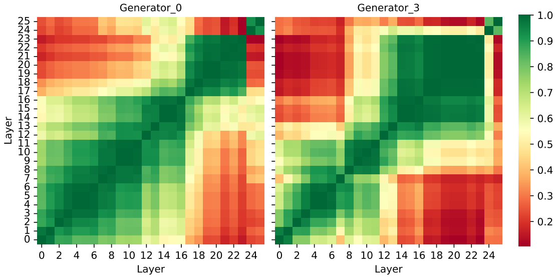
Fig. 2: The search process of DONAS-GAN obtaining diverse architectures.
