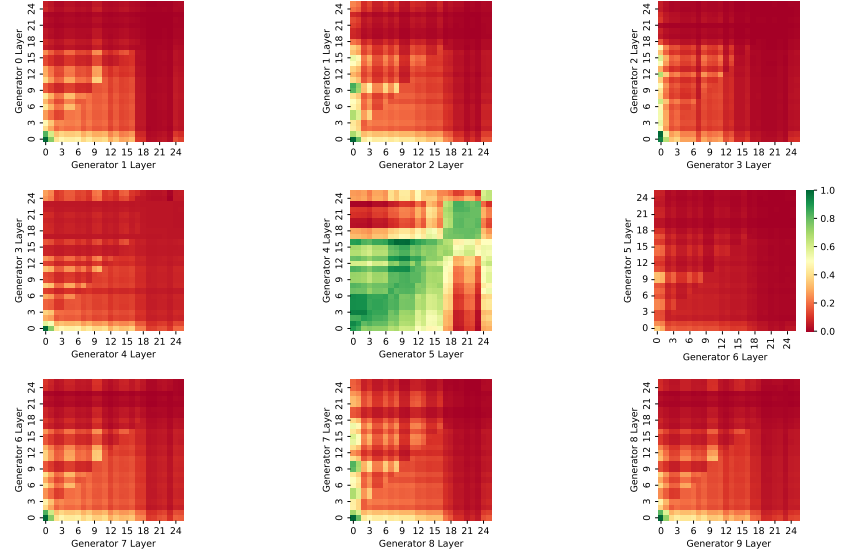
Fig. 4: Linear CKA between layers of searched generator networks by DONAS-GAN for TinyImageNet dataset.
