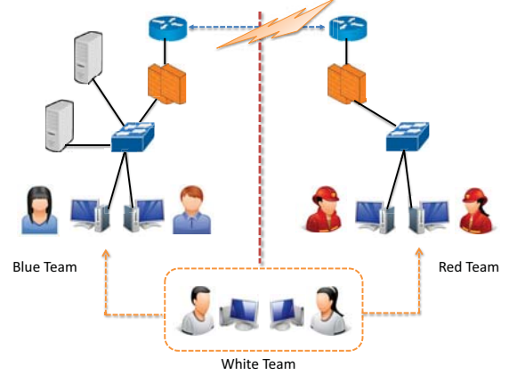
Fig. 1: Architecture of a cyber range environment.
