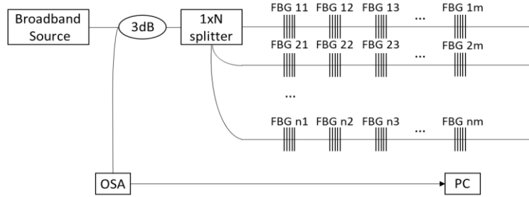
Fig.1. Schematic diagram of FBG network. OSA: optical spectrum analyzer; PC: personal computer.
