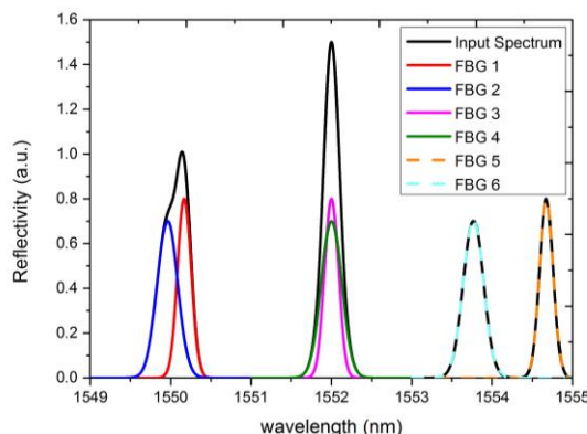
Fig.2. Testing of overlapping spectra under three typical situations
