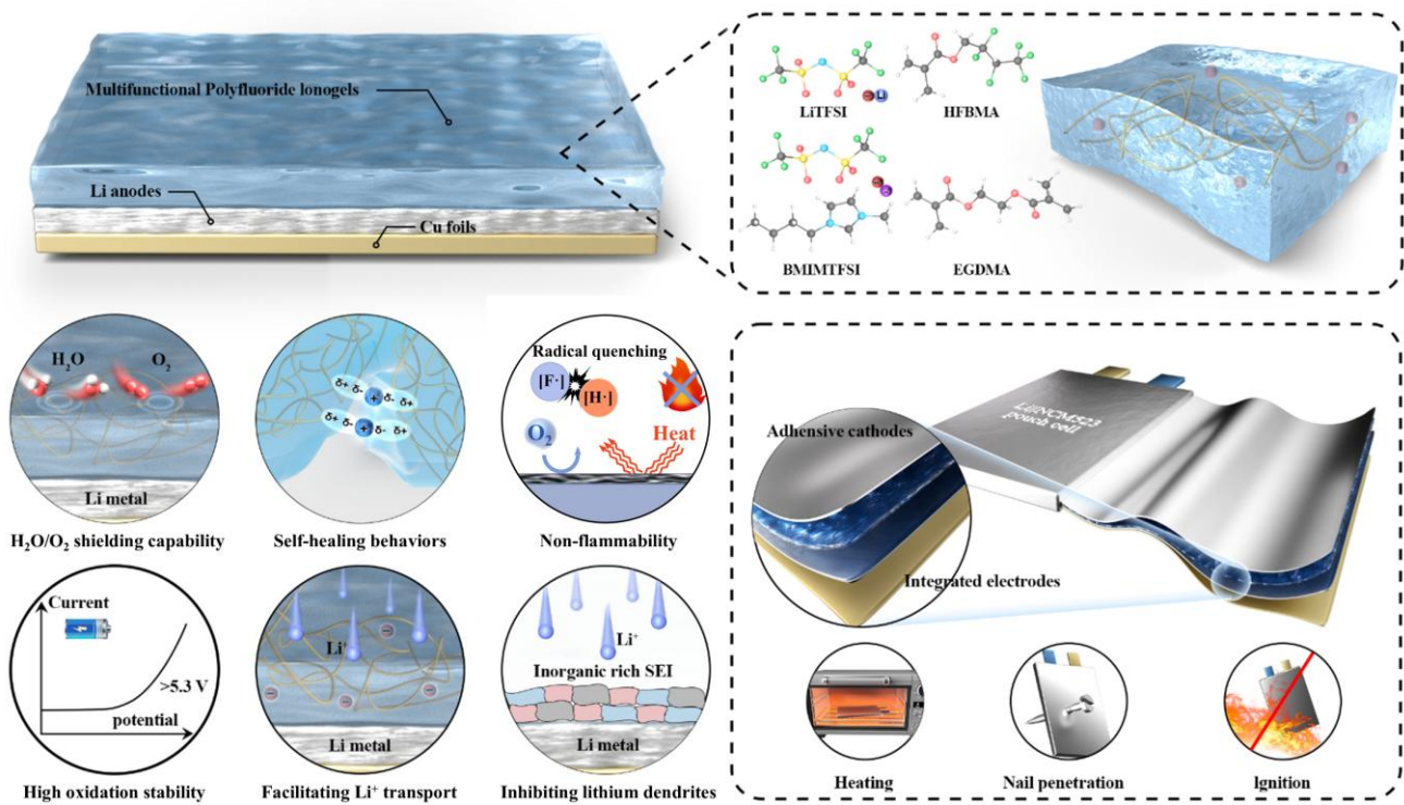
Fig. 1. Schematic illustration of the multifunctional polyfluoride ionogel-encapsulated lithium anodes. The PFIGE, with its well-designed multi-component structure, exhibits multiple advantageous properties including water/oxygen shielding capability, self-healing behavior, non-flammability, and high oxidation stability. Moreover, it facilitates \text{Li}^+ transport while effectively suppressing lithium dendrite growth. In the pouch cell design, the integrated PFIGE-encapsulated lithium anode was directly laminated with the cathode, demonstrating excellent safety performance by successfully passing rigorous heating, nail penetration, and ignition tests.
