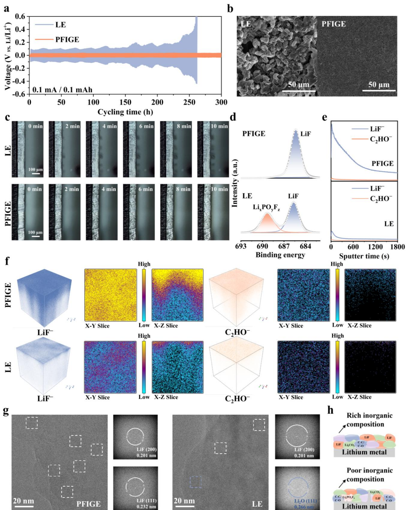
Fig. 6. (a) Cycling performance of Li||Li cells using LE and PFGE. (b) SEM images of cycled Li using LE and PFGE-based cells. (c) In-situ observation of the morphological evolution of electrodeposited Li under a current density of 0.5 \text{mA cm}^{-2} with different electrolytes. (d) XPS spectra corresponding to F 1s of Li metal after cycling of Li||Li cells using different electrolytes. (e) TOF-SIMS depth profiles of selected fragments on the SEI after cycling. (f) TOF-SIMS 3D spatial distribution of \text{LiF}^- and \text{C}_2\text{HO}^-
