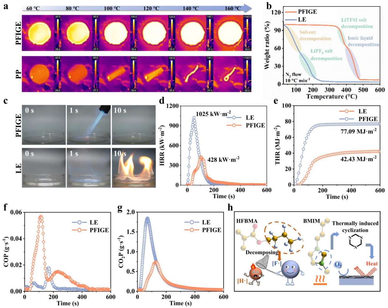
Fig. 4. (a) Infrared thermographic information of PP separators and PFIGE at different temperatures. (b) TG curves for LE and PFIGE. (c) Combustion tests of LE and PFIGE. (d) HRR, (e) THR, (f) COP and (g) CO 2 P curves of LE and PFIGE during combustion. (h) Flame-retardant mechanism of PFIGE.
