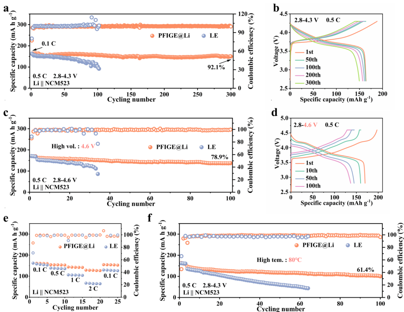
Fig. 7. (a) Cycling performance for Li||NCM523 cells using with LE and PFIGE@Li at 0.5 C. (b) Charge/discharge curves of PFIGE@Li||NCM523 cell. (c) Cycling performance of Li||NCM523 cells at 4.6 V. (d) Charge/discharge curves of PFIGE@Li||NCM523 cell at 4.6 V. (e) Rate performance of Li||NCM523 cells with LE and PFIGE@Li. (f) Cycling performance for Li||NCM523 cells with LE and PFIGE@Li at 80 °C.
