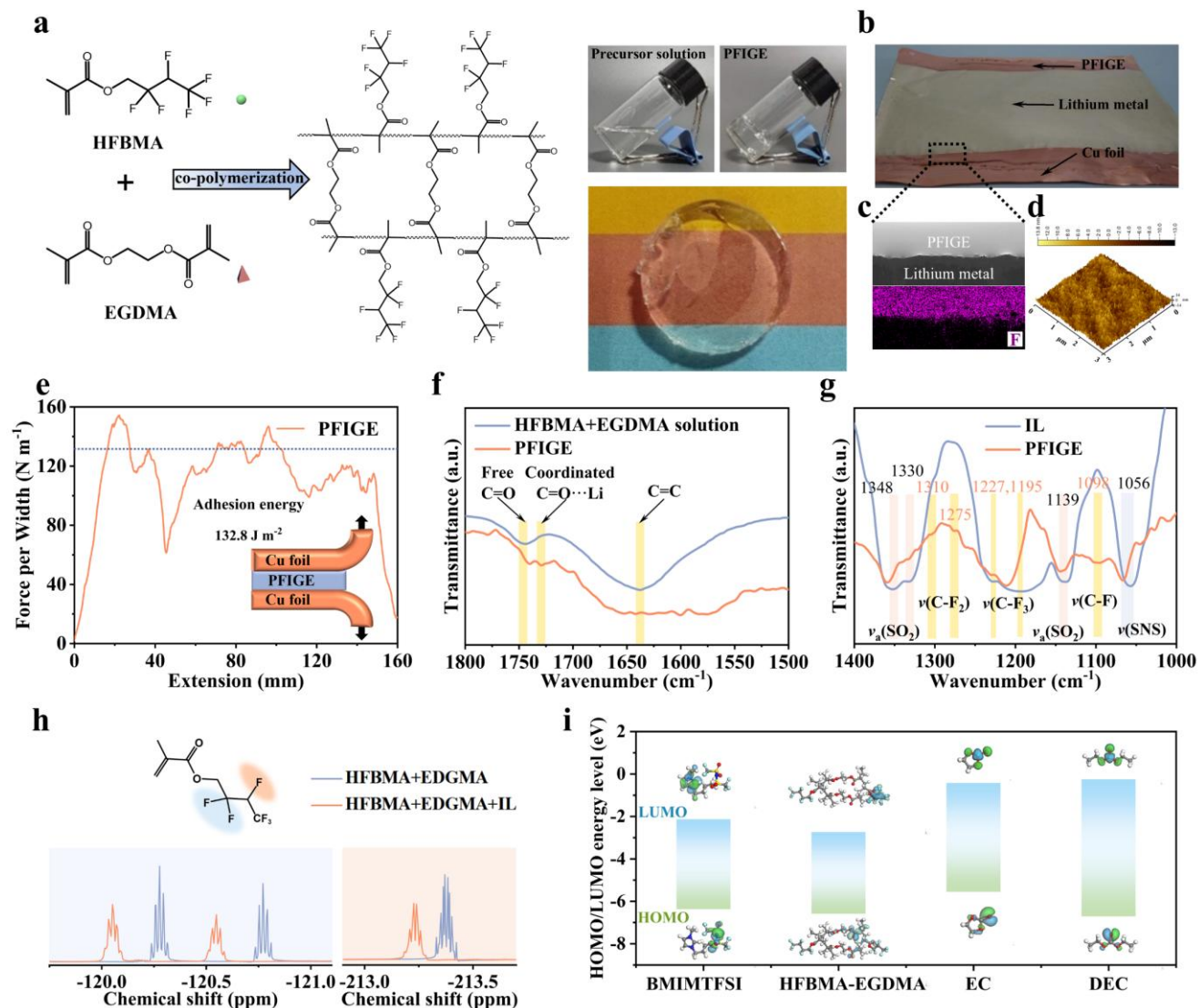
Fig. 2. (a) Synthesis of PFIGE by chemical reaction of HFBMA and EGDMA, and optical photographs before and after synthesis, and demolding. (b) Photograph of PFIGE@Li. (c) Cross-sectional image of PFIGE@Li and cross-section mapping analysis. (d) AFM images of the PFIGE. (e) Interfacial adhesion test between the PFIGE and Cu foil. (f) and (g) FTIR spectra of HFBMA+EGDMA, PFIGE, and IL. (h) 19 F NMR spectra of model samples of HFBMA+EGDMA, and HFBMA+EGDMA+IL. (i) HOMO and LUMO energy levels of BMIMTFSI, HFBMA-EGDMA, EC and DEC.
