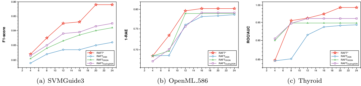
Figure 5: Model converge with other reinforcement learning method as backbone.
