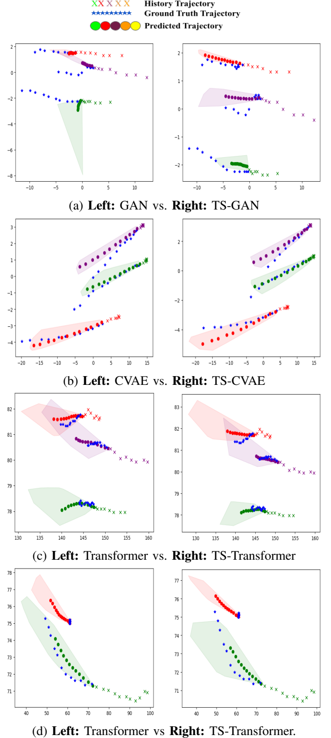
Fig. 3: Traffic State makes (a) GAN, (b) CVAE, and (c) Transformer predict more accurate mean trajectories that are closer to the ground truth. Lightly shaded areas represent the convex hull of 20 sampled trajectories. TS-based networks have tighter hulls compared to the non-TS networks which result in lower error ( \min ADE_k ) in prediction. (d) Failure case - Predictions are not closer to ground truth when traffic state is incorporated.
