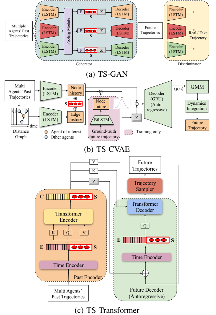
Fig. 2: Different traffic state based trajectory prediction architectures. (a) TS-GAN - traffic state S is introduced after pooling module, (b) TS-CVAE - traffic state is added to encoder output (LSTM) (c) TS-Transformer - traffic state is added to the output of both Time Encoder and Transformer Encoder. The location of traffic state insertion is empirically determined based on trajectory prediction performance in Section IV-C.
