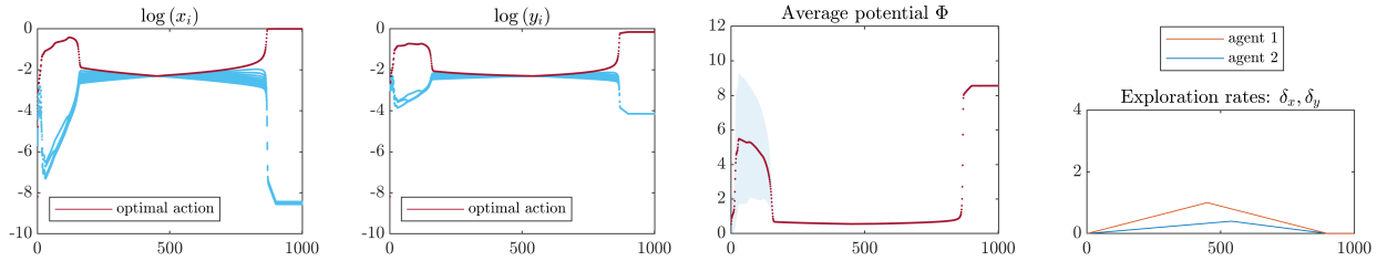
Figure 7: The SQL dynamics for the same experiment as in Figure 6 but with less intense exploration rate in the CLR-1 policies for both agents. In this case, the SQL dynamics converge to a suboptimal outcome after the exploration phase (the mean lies at 8.559 instead of the absolute maximum 10).
