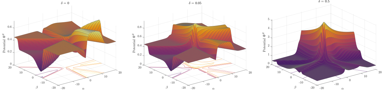
Figure 10: Snapshots of the modified potential \Phi^H for different exploration rates in a symmetric 2-player potential game with random payoffs in [0, 1] . Unlike Figures 3 and 4, we now visualize the potential function instead of the QRE surface. Hence, we cannot reason about the bifurcation types. However, we see that without exploration, \delta = 0 , the potential (equal to the potential, \Phi , of the original game) has various local maxima, whereas as exploration increases, a unique remaining attractor (maximum) forms at the vicinity of the uniform distribution, i.e., the (0, 0) point in the transformed coordinates.
