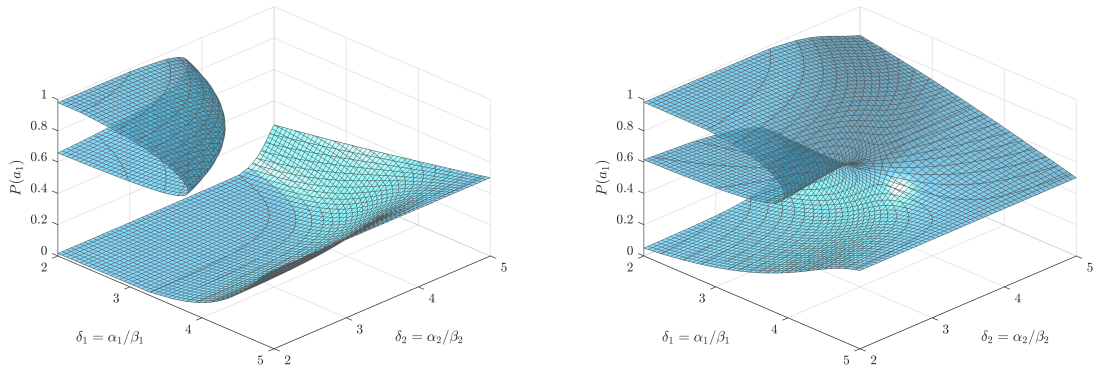
Figure 1: Geometry of QRE surfaces: single saddle-node bifurcation curve (left) vs two branches of saddle-node bifurcation curves meeting which is consistent with the emergence of a co-dimension 2 cusp bifurcation (right) on the QRE manifold of two-player, two-action games as function of the exploration rates, \delta_x, \delta_y (cf. Figures 3 and 4 for more details). The possible learning paths before, during and after exploration depend on the geometry of the QRE surface (Theorems 4.1,4.3).
