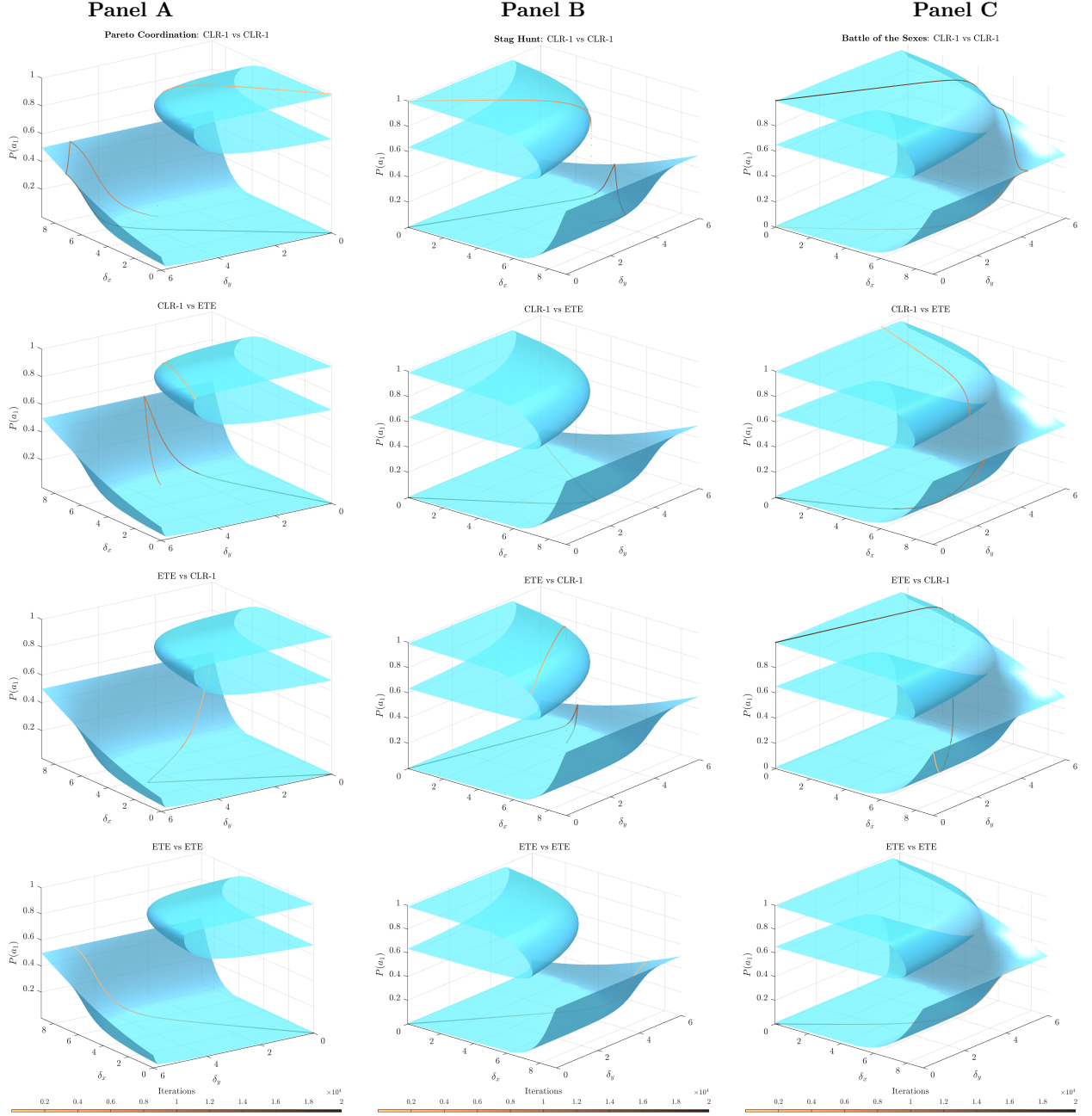
Figure D.11: SQL dynamics ( 1e+03 Q-value updates for each of 2e+04 choice distribution updates) with the ETE and CLR-1 policies in coordination games. In Pareto Coordination (Panel A) and Stag Hunt (Panel B), the SQL dynamics converge to the risk dominant equilibrium regardless of the starting point ( saddle-node bifurcations ). By contrast, in the Battle of the Sexes (Panel C), the collective outcome of the exploration process is a priori ambiguous, and the SQL dynamics may converge to either of the pure action equilibria (consistent with cusp bifurcations ). The decisive feature is the geometry of the QRE surface, i.e., whether it is connected or not, as formalized in Theorems 4.1 and 4.3.
