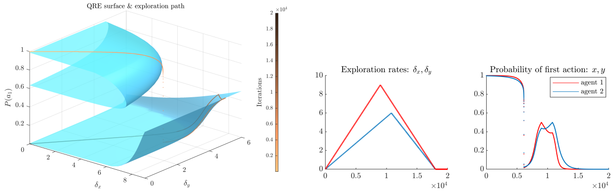
Figure 3: SQL in Stag Hunt. The left panel shows the QRE surface and the exploration path of agent 1 (light to dark line). The right panels show the CLR-1 exploration rates (left) and the probability of action 1 during the learning process for both agents. As agents increase exploration, their choice distributions undergo a saddle-node bifurcation (disconnected surface). This prompts a permanent transition from the vicinity of the payoff-dominant action profile, (a_1, a_1) , in the upper component of the QRE surface to the (a_2, a_2) equilibrium when exploration reduces back to zero (right corner of the lower component). A top-down view of the QRE surface is provided in the left panel of Figure 5.
