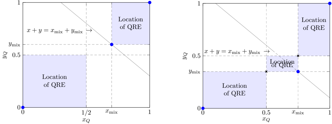
Figure 2: Geometric locus of QRE in 2 \times 2 coordination games for all possible exploration rates in the two cases (i) x_{\text{mix}} > 0.5, y_{\text{mix}} \geq 0.5 (left panel) and (ii) x_{\text{mix}} > 0.5, y_{\text{mix}} < 0.5 (right panel) of Theorem 4.3. The NE of the underlying game \Gamma (when exploration is zero) are denoted with blue dots. In the right panel, the black cross marks denote the two connecting QREs at (0.5, y_{\text{mix}}) and (x_{\text{mix}}, 0.5) . In both panels, the risk-dominant equilibrium is (0, 0) .
