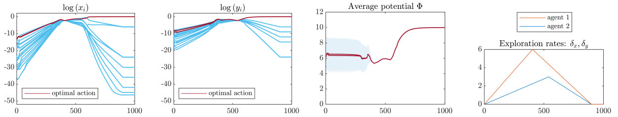
Figure 8: Exploration-Exploitation with the SQL dynamics in a potential game with n = 10 actions and a global maximum payoff of 10. The panels are as in Figure 6 and again show averages over a 10 \times 10 grid of starting points, each of which is close to one pure action profile.
