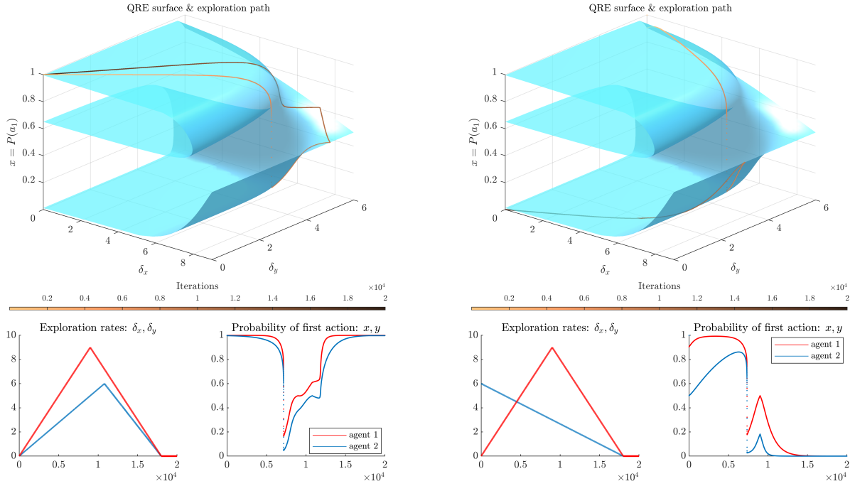
Figure 4: Exploration-Exploitation in Battle of the Sexes. In contrast to Stag Hunt, the QRE manifold has two branches of saddle-node bifurcation curves (consistent with the emergence of a co-dimension 2 cusp point) and the phase transition to the lower part of the QRE surface may not be permanent. These two cases are illustrated via the CLR-1 vs ETE policies (left) and the CLR-1 vs CLR-1 policies (right). A top-down view of the QRE surface is provided in the right panel of Figure 5.
