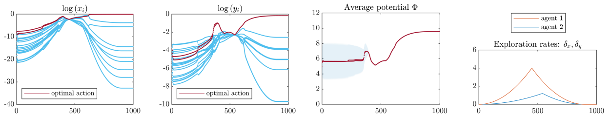
Figure 9: The game and panels are as in Figure 8. Agent 2 reduces their exploration rate in comparison to Figure 8 (fourth panel; also note the quadratic increase-decrease in the exploration rate). The SQL dynamics converge to a suboptimal state with potential value 9.561 (flat line in the right part of the third panel) for all trajectories (even for those initially close to the global optimum) as can be inferred by the vanishing shaded region (one standard deviation).
