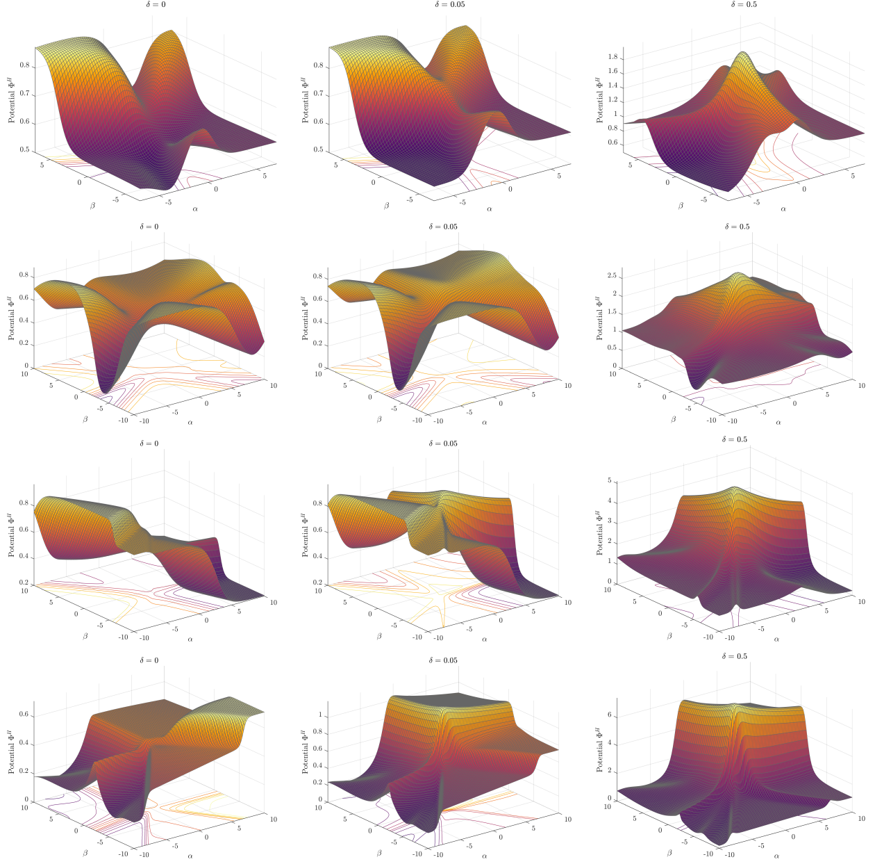
Figure D.12: From top to bottom: snapshots of the modified potential \Phi^H surface in 2 player potential games with n = 4, 10, 100 and 1000 actions, respectively, and random payoffs in [0, 1] . The surfaces are plotted using Algorithm 1 (see [42]). From left to right: the exploration rate \delta increases from \delta = 0 to \delta = 0.05 and \delta = 0.5 . The surface has arbitrary maxima (resting points of the SQL dynamics) when \delta is small (exploitation) but a single maximum at (or close to) (0, 0) which corresponds to the uniform distribution when \delta is large (exploration). Intuitively, this is what agents see as they increasingly incorporate exploration in their utilities.
