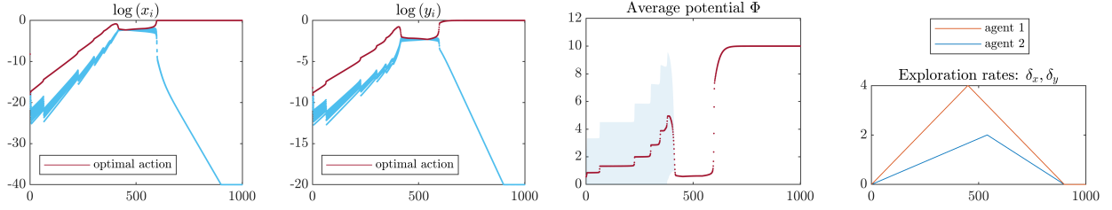
Figure 6: SQL dynamics ( 1e + 20 Q-value updates for each of 1e + 03 choice distribution updates) in a pure coordination game with n = 10 actions and diagonal payoffs u_{ii} = i for i = 1, \dots, 10 , cf. equation (8). The first two panels show the (log) choice distributions (with the optimal action in different color). The third panel shows the average potential over a set of 10 \times 10 different trajectories (starting points) and one standard deviation (shaded region that disappears after all trajectories converge to the same choice distribution). The fourth panel shows the selected CLR-1 policies. Both agents perform CLR-1 exploration with different intensities and all trajectories of the SQL dynamics converge to the global optimum after the exploration phase regardless of the starting point (the standard deviation, depicted as the shaded region in the third panel, vanishes).
