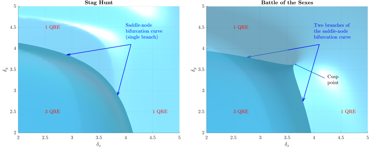
Figure 5: QRE surfaces in Stag Hunt (left panel) and Battle of the Sexes (right panel). The depicted surfaces are the same as in Figures 1, 3, 4 and D.11. The current perspective is from the top of the z-axis. The x-y axes have been set between 2 and 5 for a better focus on the bifurcation curve. 360° rotations of these surfaces are shown in the online supplementary material.
