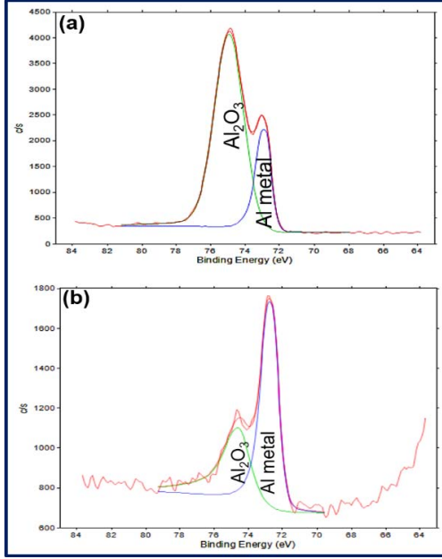
Figure 5. XPS spectra of Al2p core level analysis of Al surface with, (a). no passivation layer. (b). 2nm Ti passivation.
