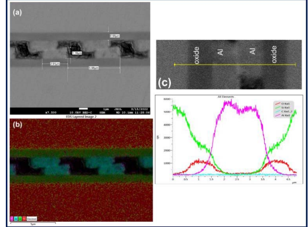
Figure 7. (a) The X-SEM image of the fine pitch bonded interface. (b). The EDS elemental areal map of the bonded wafers. (c). The EDS line scan across the bonded interface.
