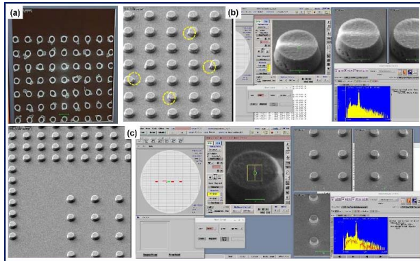
Figure 6. The DR-SEM inspection of Al patterns with passivation layer, (a). The surface after PR strip off. (b). pits on the edges (circled in yellow label) with EDS on respective pattern. (c). The clear pattern with respective surface EDS scan.
