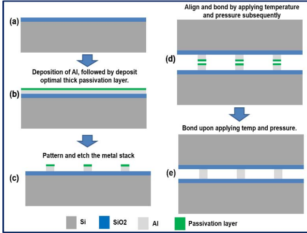
Figure 1. Process flow for the fine pitch aluminum-aluminum bonding.
