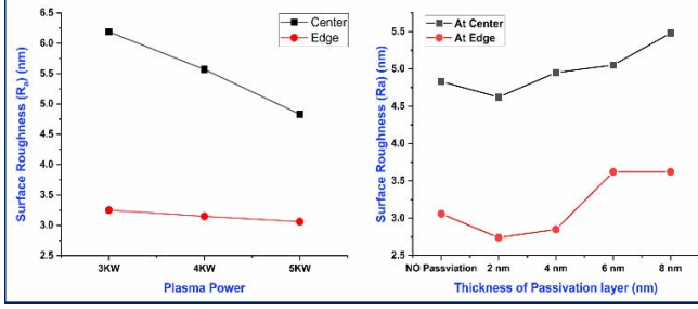
Figure 2. The resulted average surface roughness ( 5\mu\text{m} \times 5\mu\text{m} area). (a). On the Al surface with varying the plasma power. (b). By varying the passivation layer thickness.
