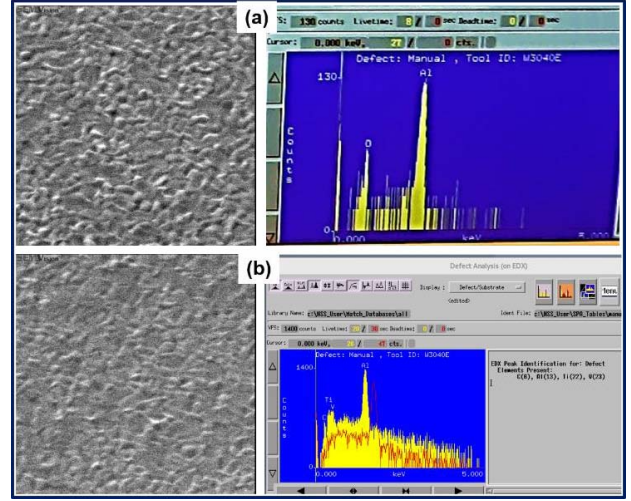
Figure 4. The energy dispersive spectroscopy areal scan on, (a). the surface of Al without passivation layer. (b). On the surface of the thin Ti passivated Al surface.
