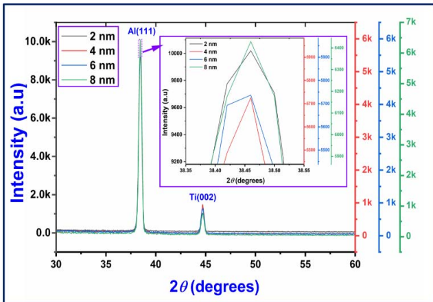
Figure 3. The grazing angle XRD inspection of Al surface with varying passivation layer thickness.
