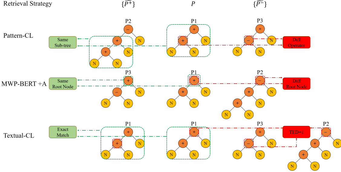
Figure 1: Triplets construction results based on different retrieval strategies.
