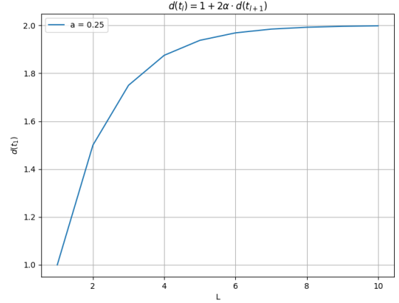
Figure 4: The simulation of the limitation in Equation 3.
