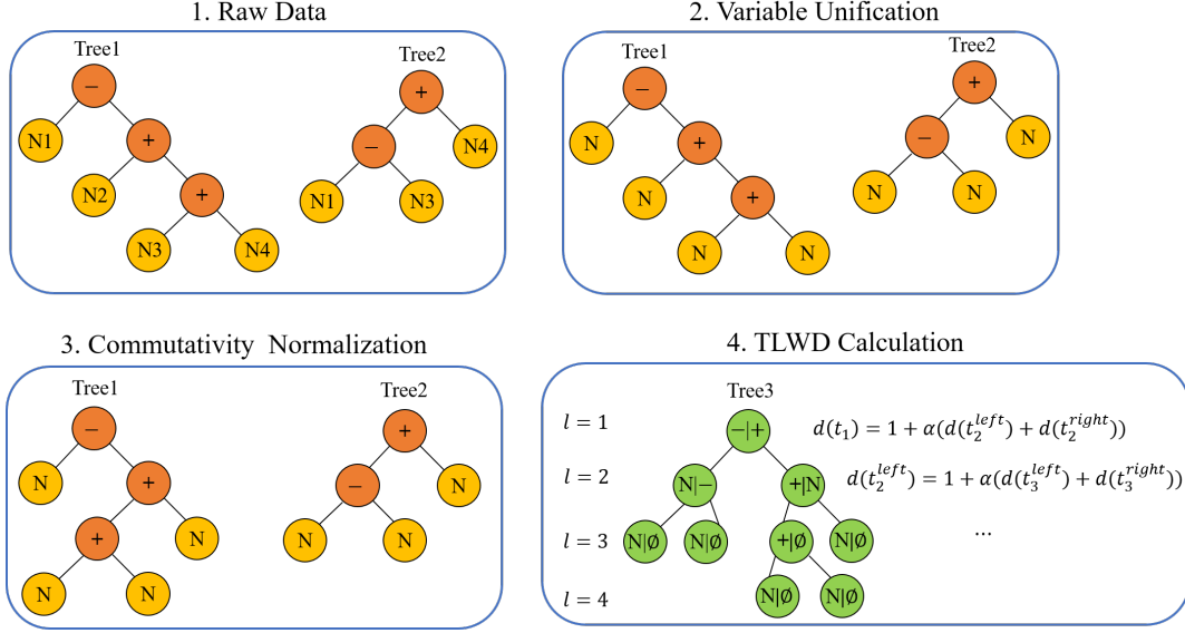
Figure 3: Overview of the TLWD Calculation procedure. Levels of the tree are defined from top to bottom. Lower levels are closer to the root and carry global information of the tree, while higher levels are towards the bottom and provide more detailed local information.
