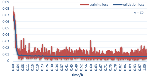
Fig. 3: Convergence of training and validation losses.
